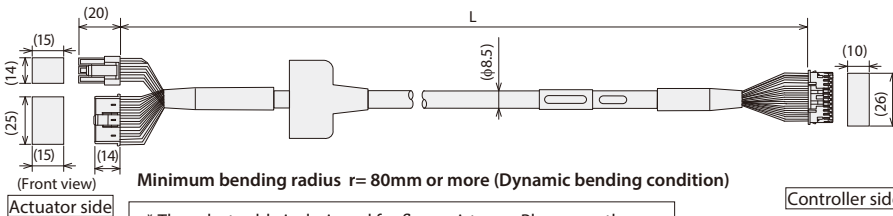
Actuator side Controller side
