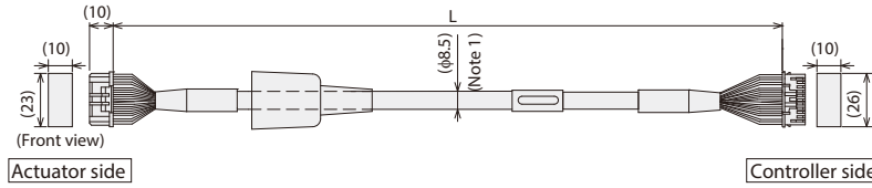
Actuator side Controller side
